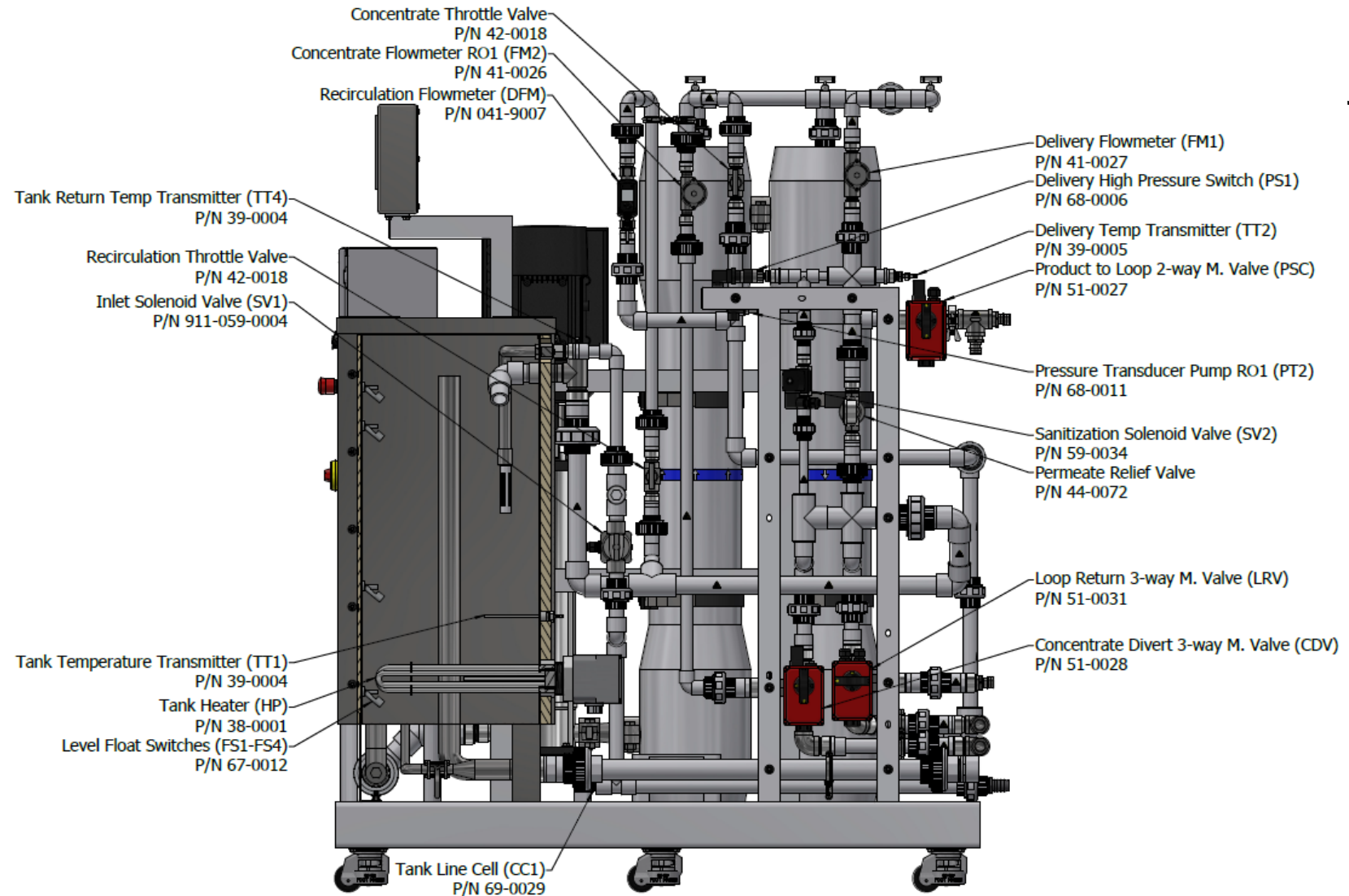
RIGHT VIEW WITH INSIDE OF BREAK TANK SHOWING
